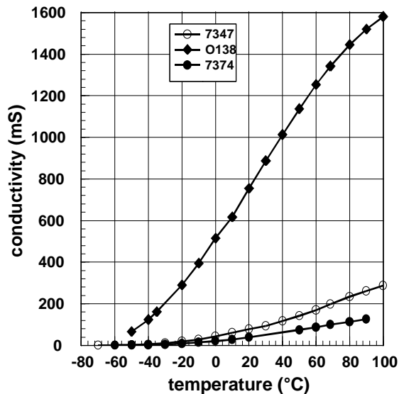
Figure 5. Conductivity vs. Temperature for various sulfuric acid based electrolytes.
