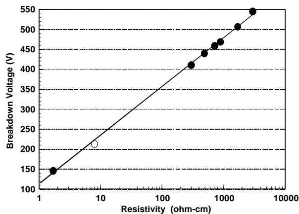
Figure 4. Breakdown voltage vs. Log electrolyte resistivity for Ta_2O_5 dielectric in various aqueous and non-aqueous electrolytes. 3
