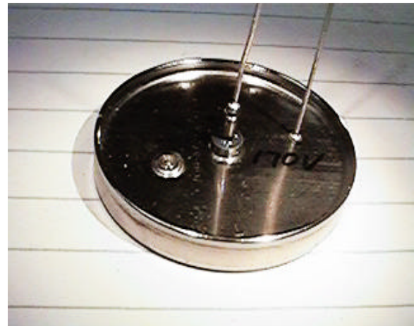
Figure 2. Photograph of the hermetic tantalum Hybrid capacitor.
