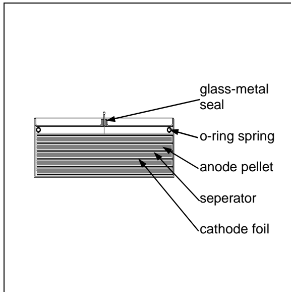
Figure 1. Schematic view showing internal construction of a multiple-anode element tantalum Hybrid capacitor.
