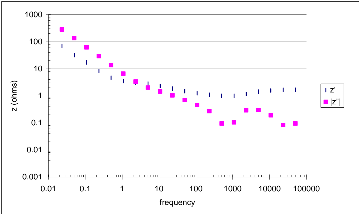
Figure 23 Impedance vs. frequency for the aluminum hybrid capacitor. The data confirm a 0.995 ohm ESR measurement at 120 Hz.
