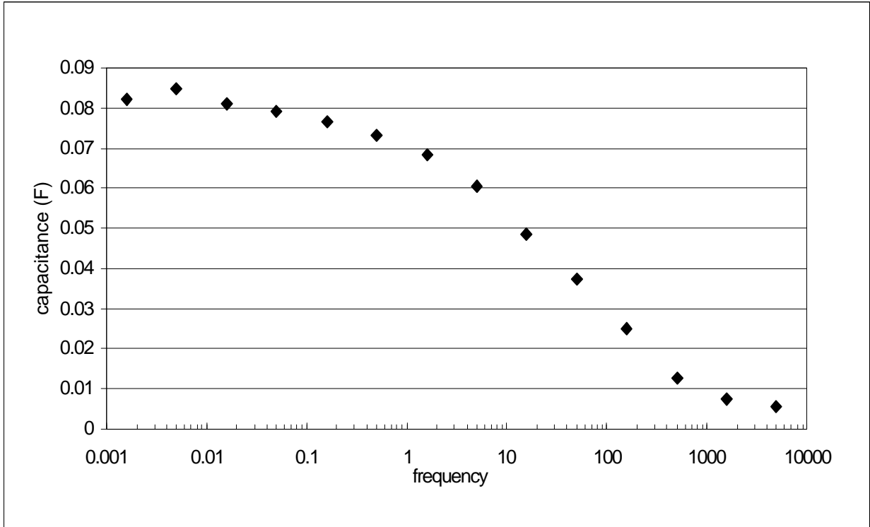
Figure 18. Capacitance vs. frequency for the shock-hardened tantalum hybrid capacitor. It is noteworthy that the “dc” capacitance is greater than twice the reported capacitance at 120 Hz.
