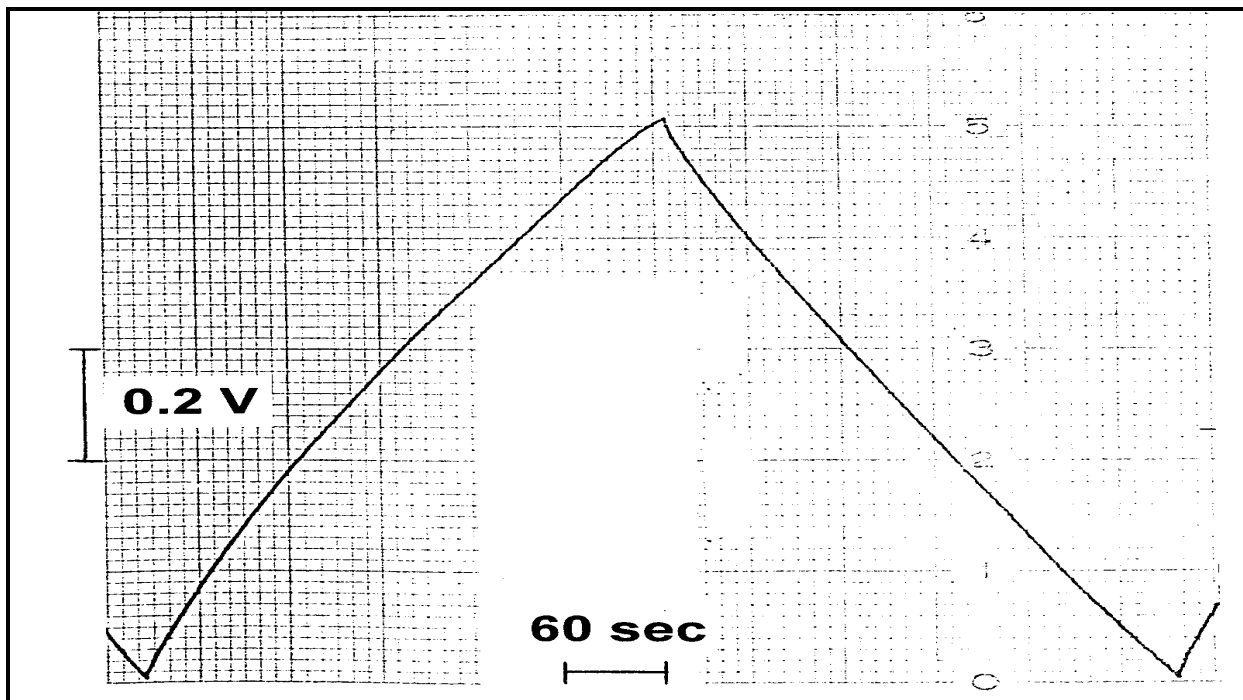
Figure 6. DC charge and discharge curve of a symmetrical capacitor with two film electrodes in H_2SO_4 electrolyte. The current was 2 mA. The voltage was 0-1 V.
