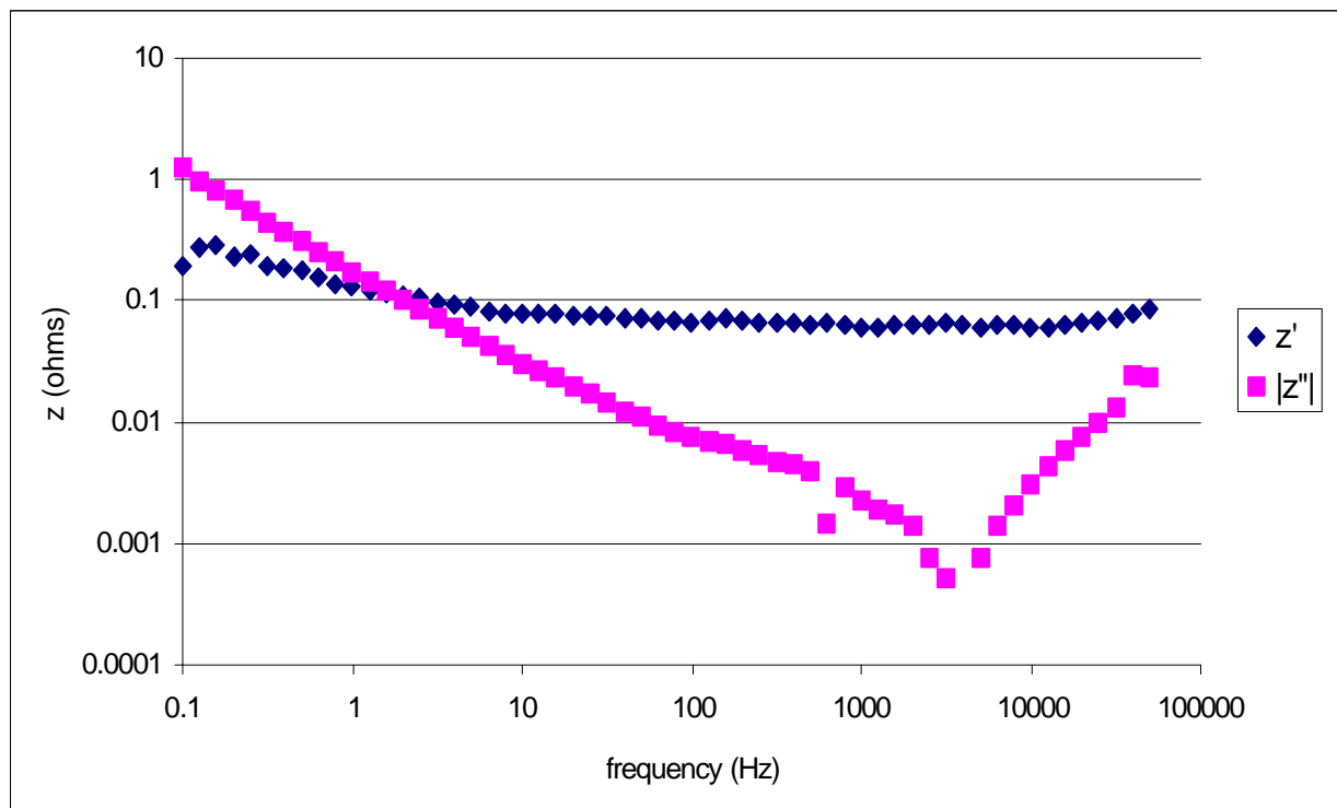
Figure 7. Electrical impedance behavior of a typical symmetric test cell using improved \text{RuO}_2 film on pre-treated tantalum foil. Note that this gives the performance of two electrodes in series. In the intended application in a hybrid capacitor where only a single electrode is needed, the impedance ( z' and z'' ) would be 1/2 the value shown.
