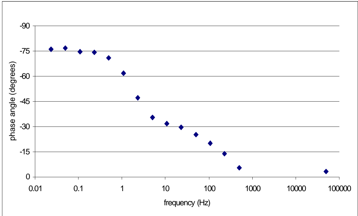
Figure 24. Phase angle vs. frequency for the aluminum hybrid capacitor. Behavior is influenced by the effects of high-resistance electrolyte.
