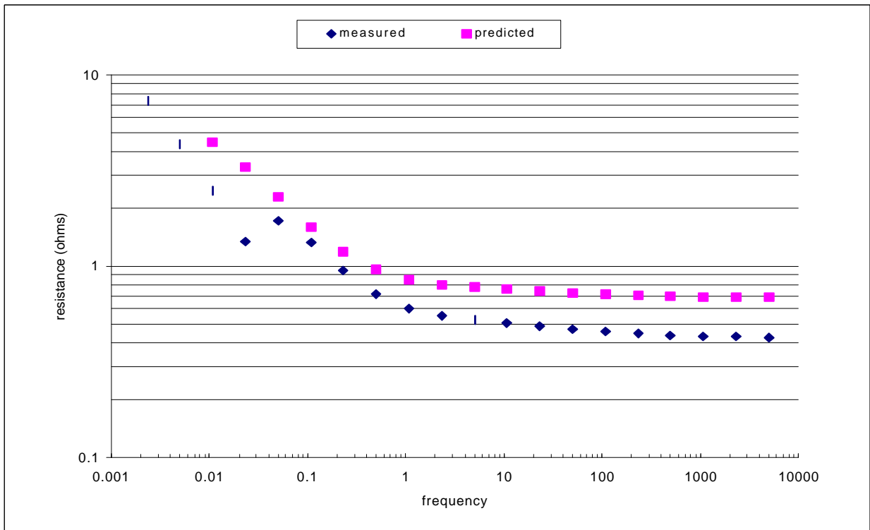
Figure 14 (above) and Figure 15 (below) show the capacitance and resistance vs. frequency for the twelve-cell symmetric particulate amorphous \text{RuO}_2 shock-hardened capacitor prototype. Predicted results are based on the average results of individual cells in a theoretical capacitor according to Ohm's Law. That the prototype capacitor performed better than predicted may be attributed to more axial compression of the cell and lower contact resistance than in the cell measurement fixture.
