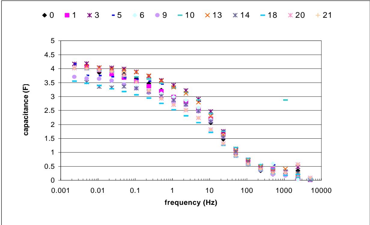
Figure 12. Capacitance vs. frequency for the twelve symmetric particulate amorphous RuO 2 cells used in the shock-hardened capacitor prototype.
