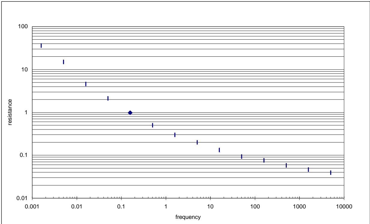
Figure 19. Resistance vs. frequency for the shock-hardened tantalum hybrid capacitor.
