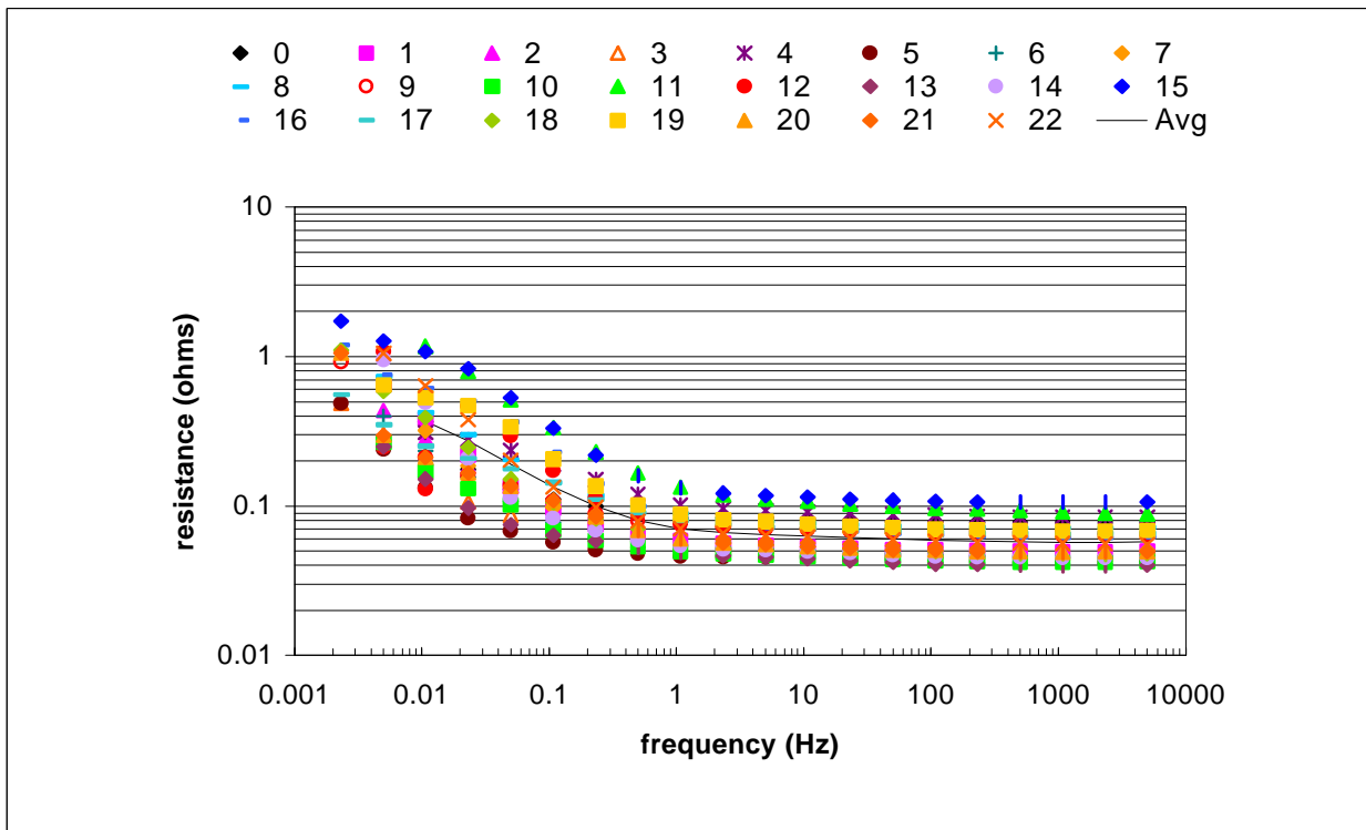
Figure 11. Resistance vs. frequency for symmetric particulate amorphous RuO 2 cells.
