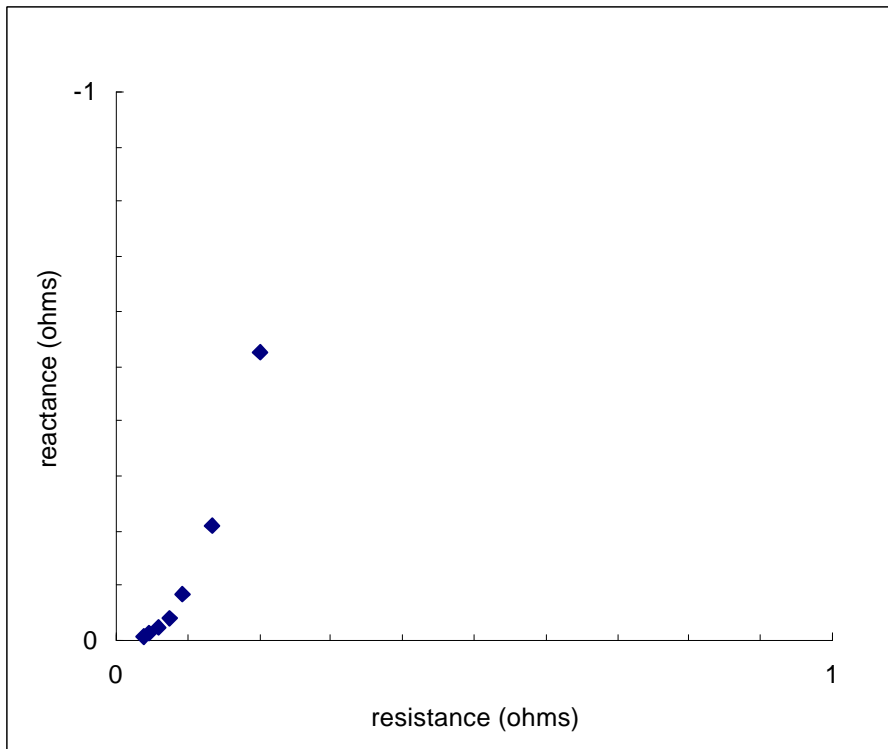
Figure 21. The figure to the right is a Nyquist plot of the impedance data. The plot intersects the x-axis at nearly 45^\circ , indicative of the use of porous electrodes.
