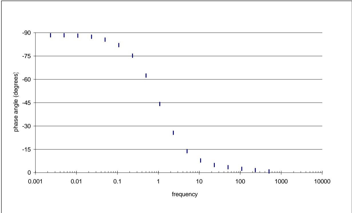
Figure 16. Phase angle vs. frequency for the twelve-cell symmetric particulate amorphous \text{RuO}_2 shock-hardened capacitor prototype.
