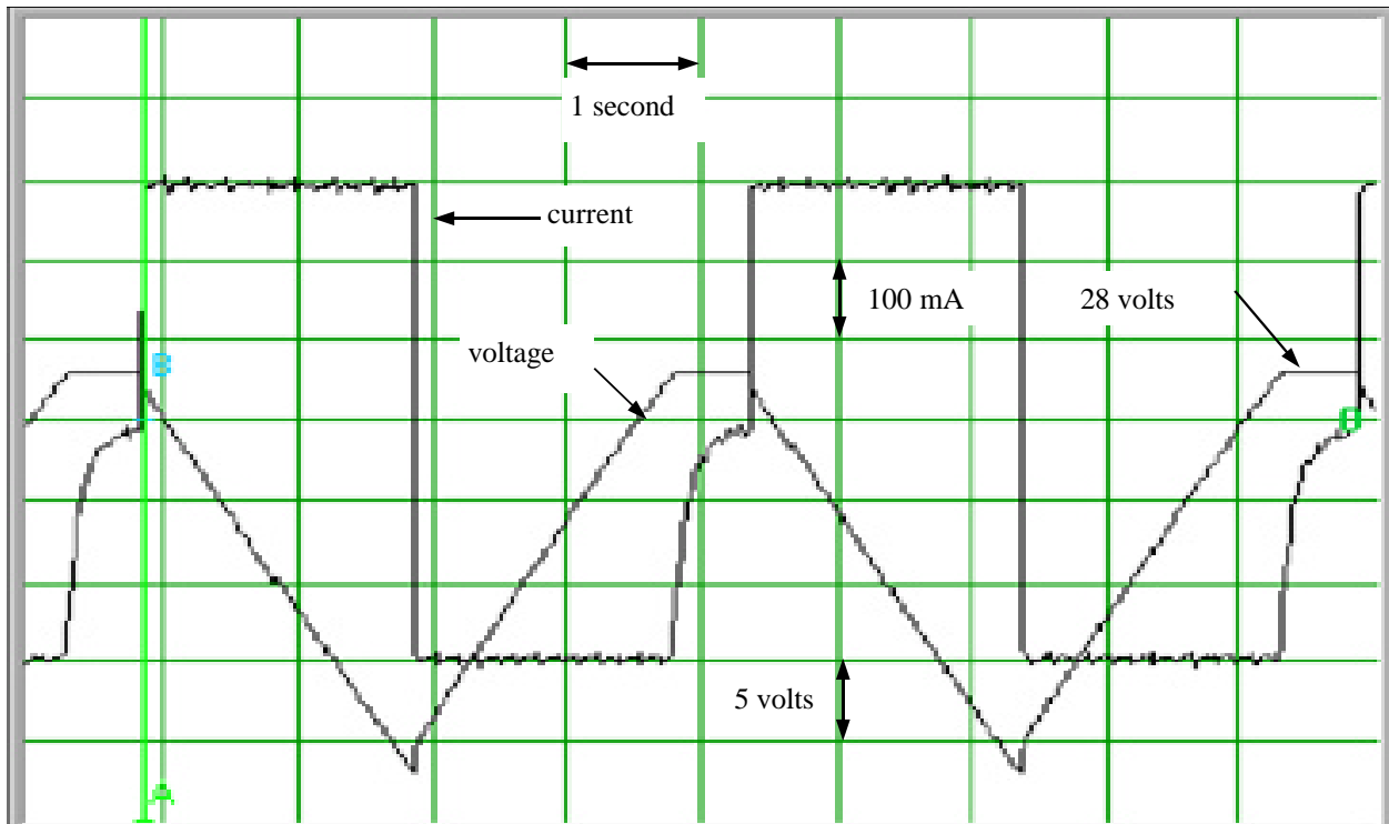
Figure 25. Charge-discharge curve for the aluminum hybrid capacitor. The data correspond to a capacitance of 0.024 F. A constant current charge / load of 300 mA was applied. The voltage cycled between 3 - 28 volts. The period is 4.5 s.
