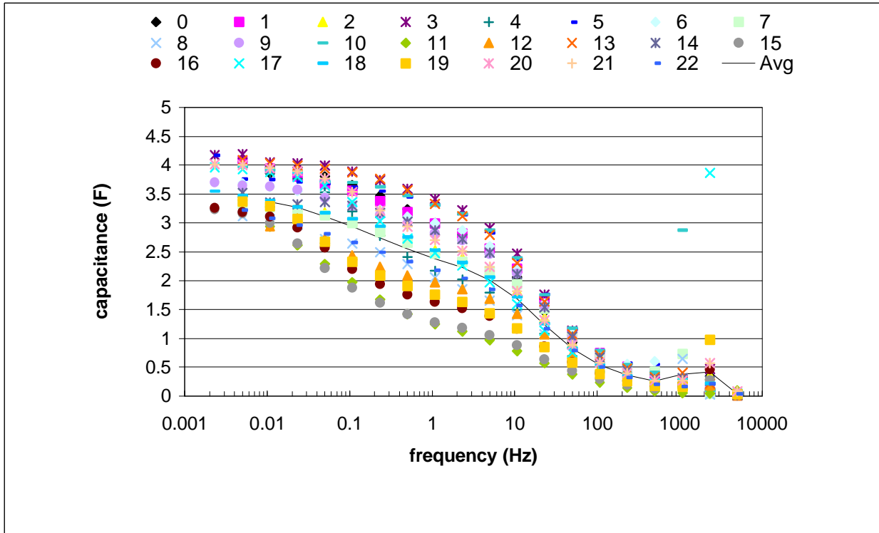
Figure 10. Capacitance vs. frequency for symmetric particulate amorphous RuO 2 cells.
