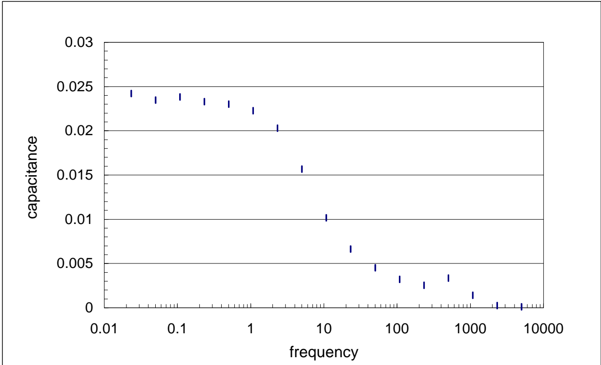
Figure 22 Capacitance vs. frequency for the aluminum hybrid capacitor. The high rate of change in capacitance with frequency has not been observed with tantalum capacitors.
