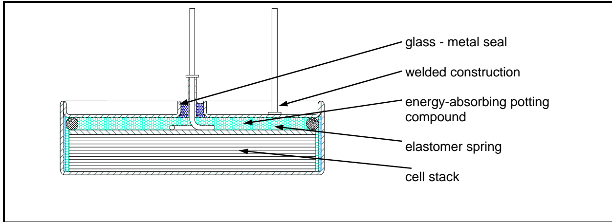
Figure 1. Drawing of the 12-cell shock-hardened symmetric amorphous RuO_2 \cdot xH_2O prototype capacitor showing details of the internal construction. Upon acceleration, small motion of the cell stack relative to the case causes the potting compound to flow. This, in turn, absorbs energy, cushioning the shock. The unit is designed to allow the motion under the influence of the elastomer spring without effecting electrical performance.
