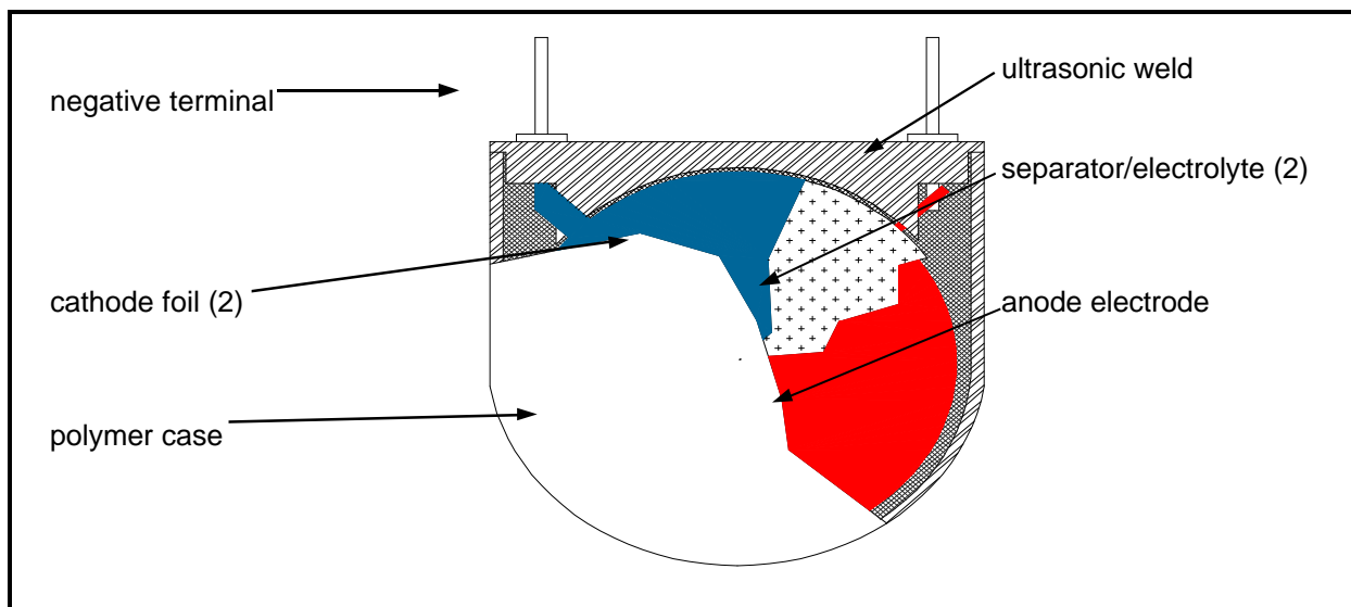
Figure 4. Cut-away view of aluminum hybrid electrochemical-electrolytic capacitor in polymer case. The packaging used is an adaptation of tantalum Hybrid® capacitor case components.
