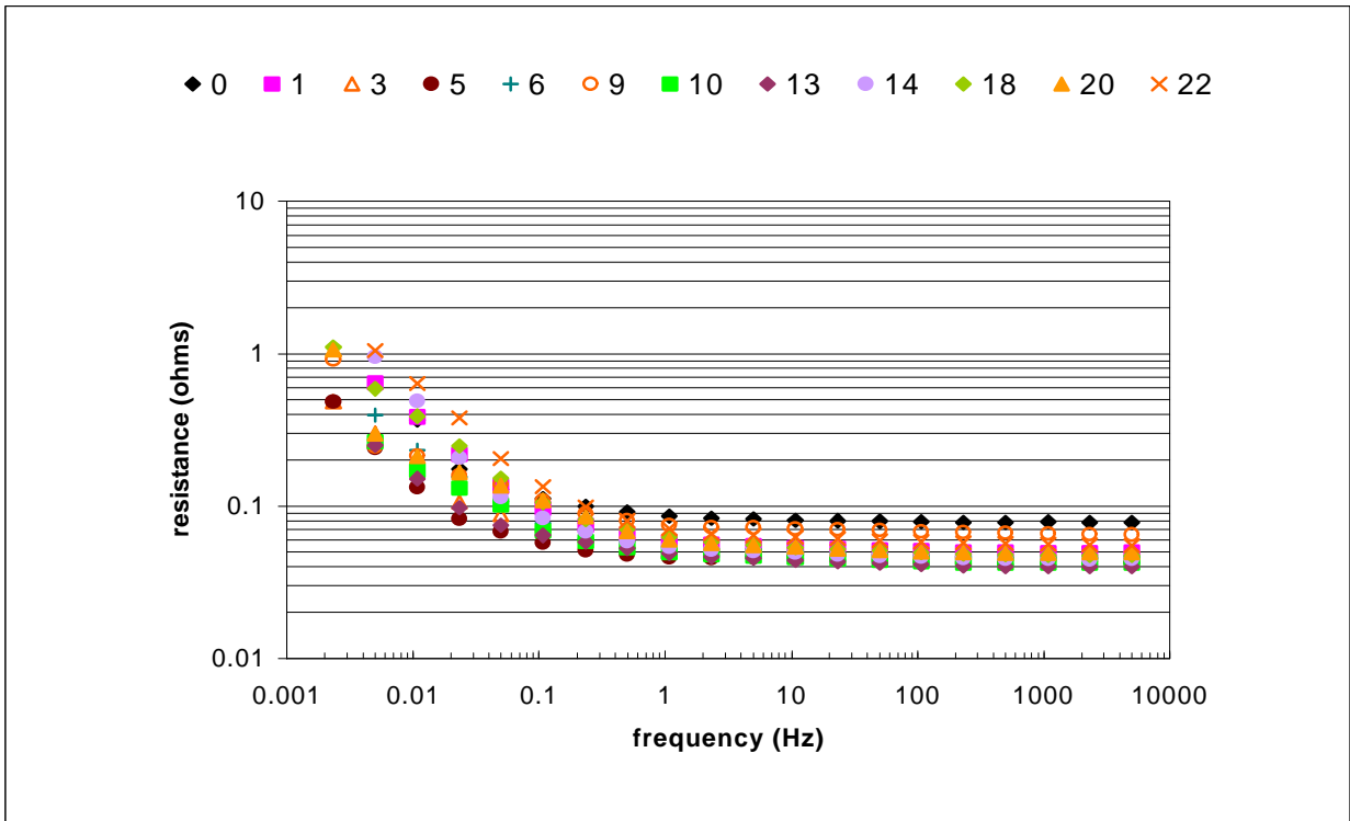
Figure 13. Resistance vs. frequency for the twelve symmetric particulate amorphous RuO 2 cells used in the shock-hardened capacitor prototype.
