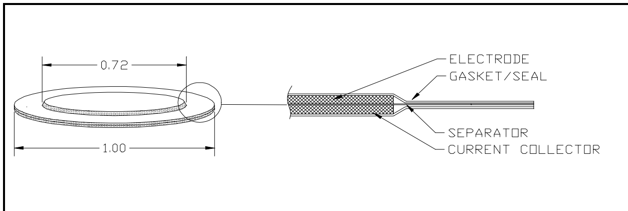
Figure 2. Cell cross-section view
