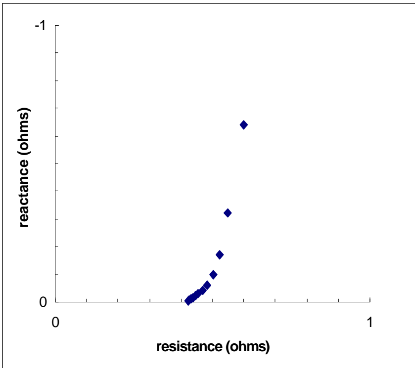
Figure 17. Nyquist plot of the impedance data for the twelve-cell symmetric particulate amorphous \text{RuO}_2 shock-hardened capacitor prototype.
