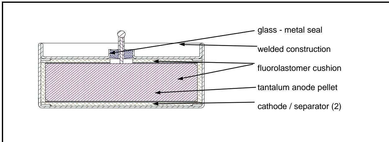
Figure 3. Drawing of the 25 V shock-hardened hermetic tantalum prototype capacitor showing details of internal construction. Upon acceleration, this unit absorbs mechanical energy due to the motion of the anode relative to the case. This motion, governed by the elastomer cushion, forces internal electrolyte flow, dissipating energy and reducing the peak load.
